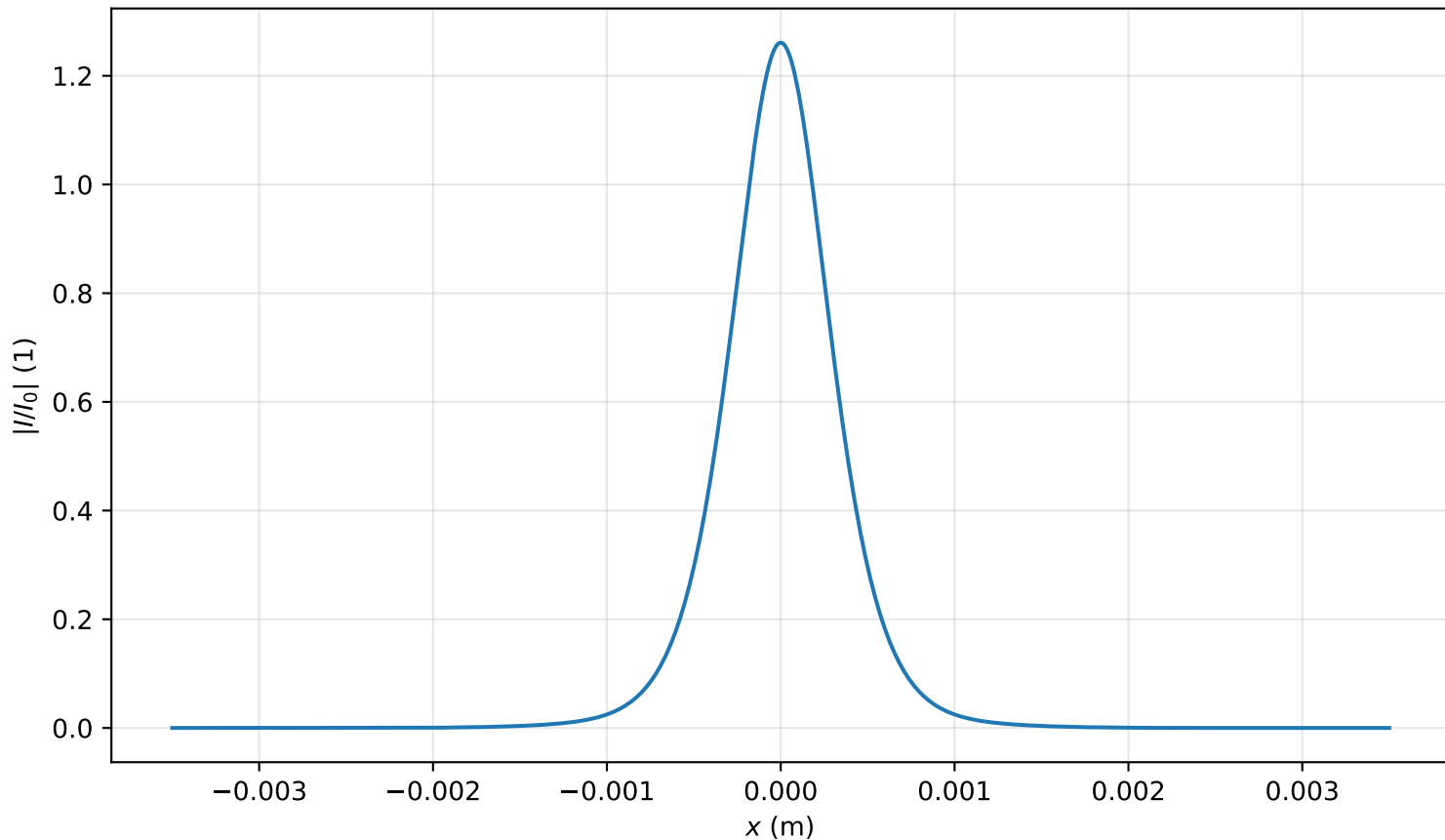
Intensity profile I(x, y = 0, z = 2.309m)/I_0 , P_{in}=0.8P_{cr} , artificial time
